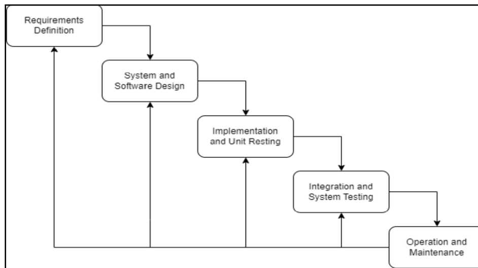
Gambar 2.1 Model Waterfall
